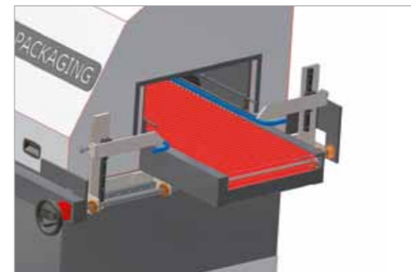
Tunnel con sponde di raffreddamento Refrigerated water cooled guides in tunnel
